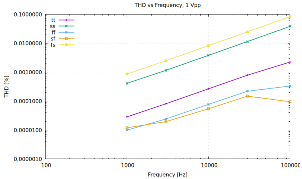
THD vs Frequency, All Corners
