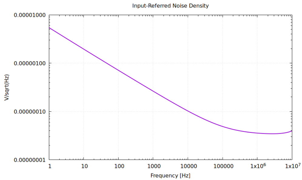
Input-Referred Noise Density vs Frequency
