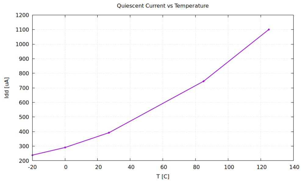
Quiescent Current vs Temperature
