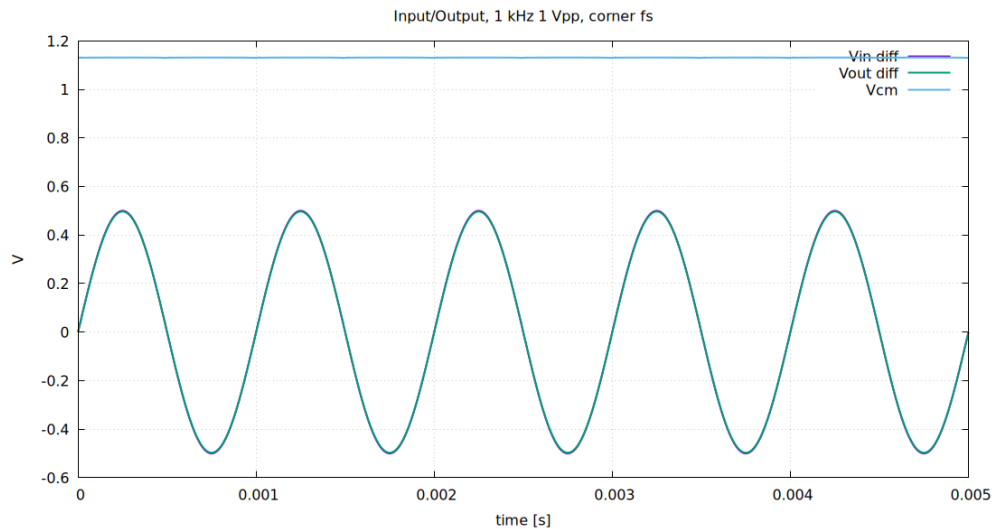
Input/Output Waveforms, fs Corner
