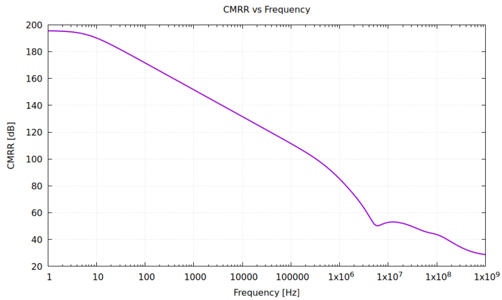
CMRR vs Frequency
