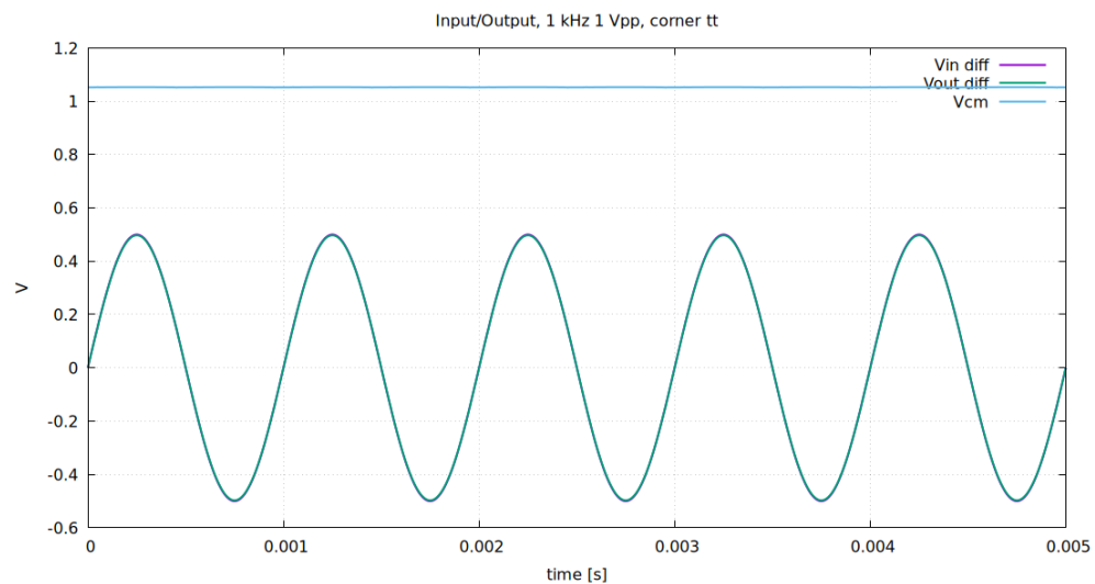
Input/Output Waveforms, 1 kHz, Unity Gain
