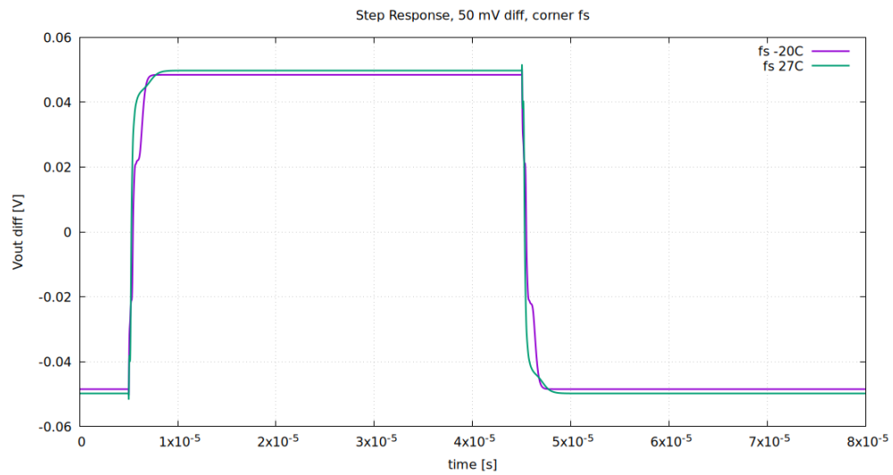
Step Response, fs Corner
