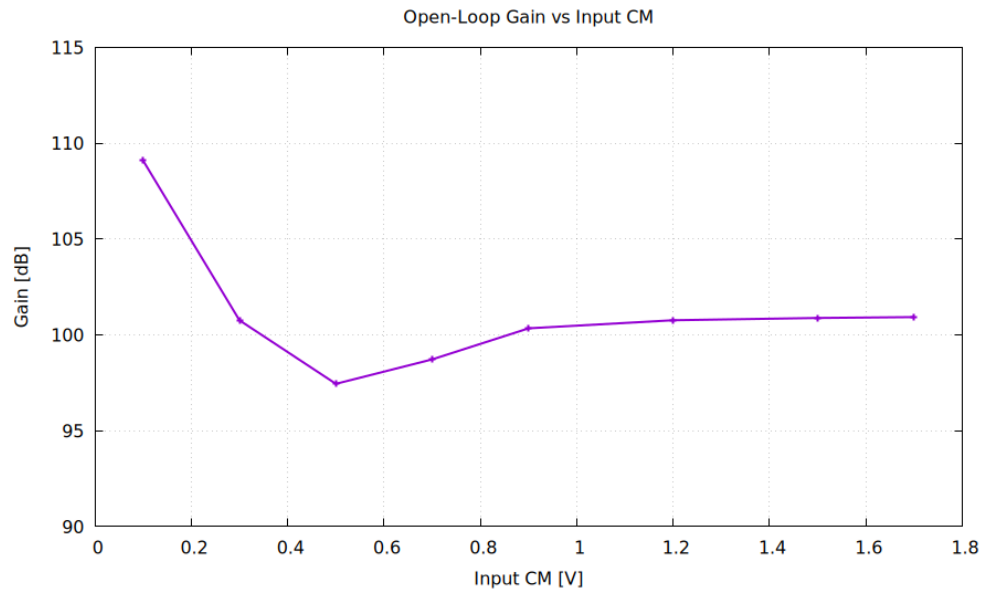
Open-Loop Gain vs Input Common-Mode
