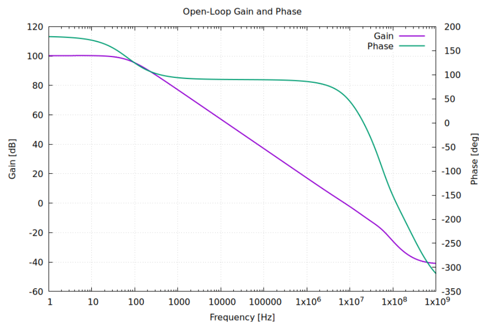
Open-Loop Gain and Phase vs Frequency
