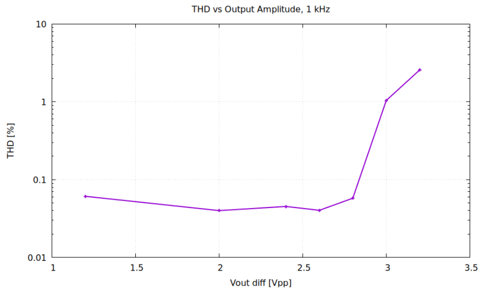
THD vs Output Amplitude at 1 kHz
