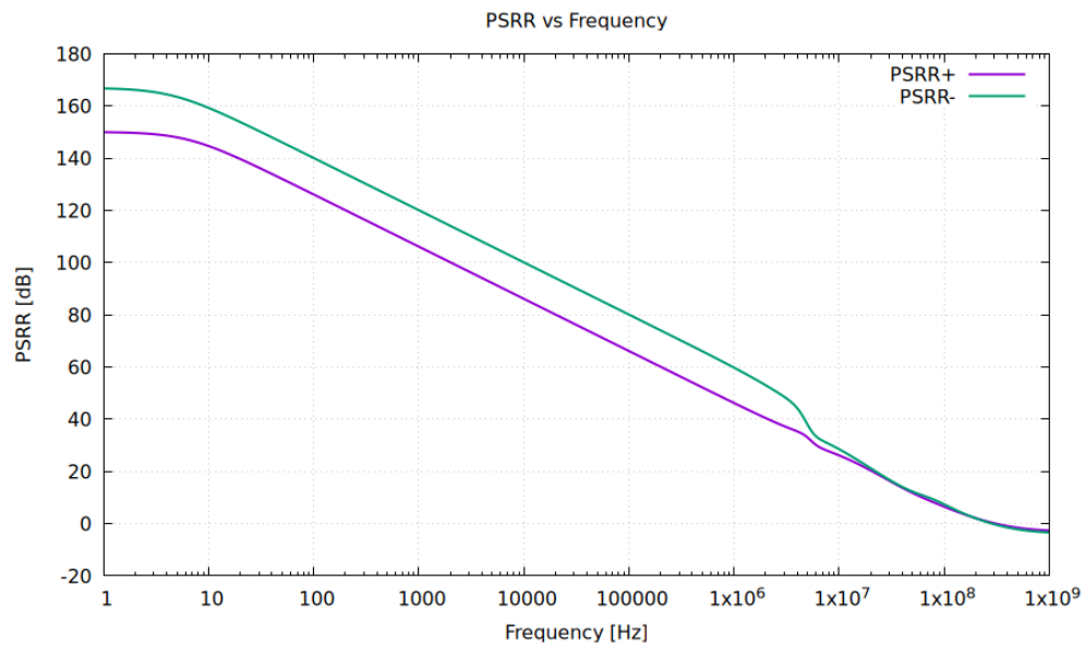
PSRR vs Frequency
