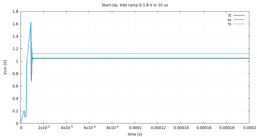
Start-Up Behaviour, Supply Ramp
